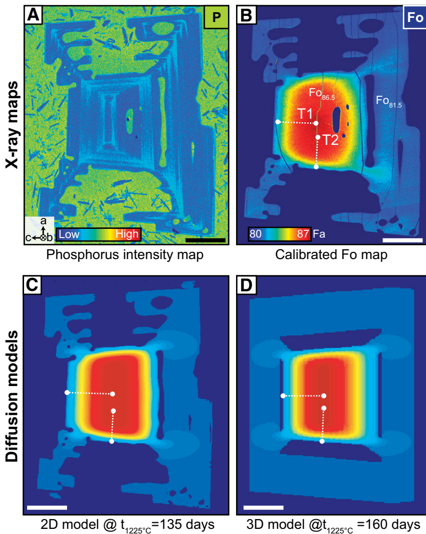
Figure 1. Comparison between zoning in a natural Kilauea olivine and best-fit two-dimensional (2-D) and 3-D diffusion models. A: Phosphorous X-ray intensity map; map preserves the initial growth history of the olivine. Small inset at bottom left shows the approximate orientation of the section with respect to the crystallographic axes. B: Fe-Mg (Fo) X-ray intensity map; map indicates a later phase of diffusive reequilibration. C, D: Best-matching 2-D and 3-D diffusion models of Fe-Mg, and corresponding time scales. The 2-D model employs the same geometry as the Fo map, whereas the 3-D model requires simplifications in the crystal shape but accounts for diffusive fluxes from all directions. Mismatches occur near the melt inclusions, which are not accounted for in the models. The section in D was sampled slightly oblique to the a-c plane to match the orientation of the natural crystal. White dotted lines show the locations of electron probe microanalysis traverses T1 and T2 used to calibrate Fo maps, and utilized as output constraints for the 2-D and 3-D models (see text for details). Scale bars represent 200 \mu\text{m} .
