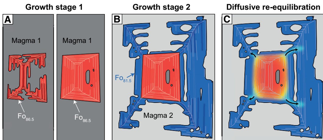
Figure 2. Interpretative petrological narrative. A: The olivine initially grows in a magma at equilibrium with a \text{Fo}_{86.5} olivine composition (red), with or without fine-scale Fo zoning (dark red), matures, and homogenizes. B: The olivine is later incorporated into a different magma olivine and grows a \text{Fo}_{81.5} skeletal rim (blue), with fine-scale Fo zoning or not (darker blue). C: The core and rim of the crystal reequilibrate diffusively for a certain period, without any significant changes in the crystal morphology. Thin white lines represent the framework marked by phosphorous zoning (see Fig. 1A).
